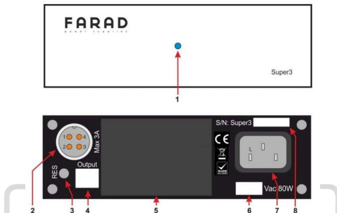
FIGURE 1: Front and back of the Super3 power supply, controls and connections
