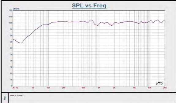
CARME-212B SPL / IMPEDANCE VS FREQ.
