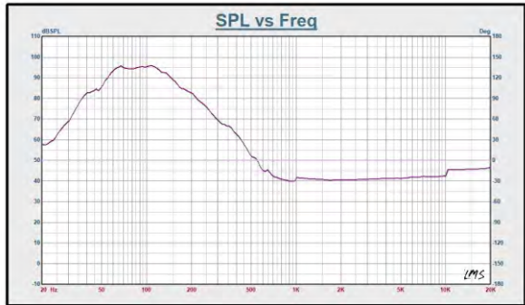
SPL / IMPEDANCE VS FREQ.
