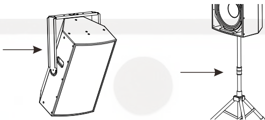
U Bracket Model: CARME-112BUBV2 (Black) CARME-112WUBV2 (White) Tripod Stand Model: STSD-71B (Black) STSD-71W (Silver)
