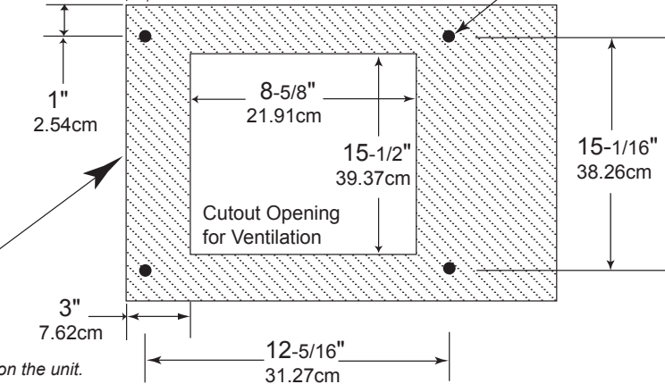
MCT500 Bottom View in Custom Cabinet
