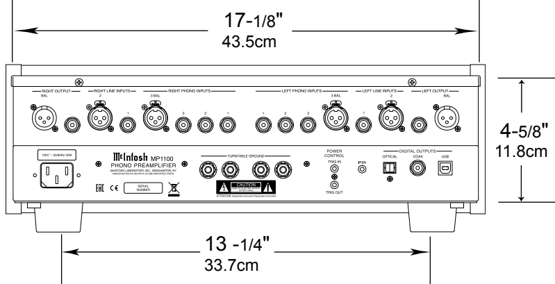
Rear View of the MP1100
