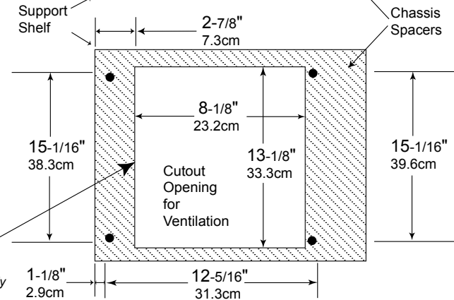
MP1100 Bottom View in Custom Cabinet
