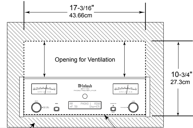
Cabinet Front Panel Cutout Opening for Custom Mounting
