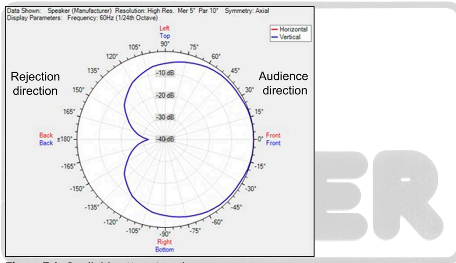
Figure 7.1: Cardioid pattern top view
