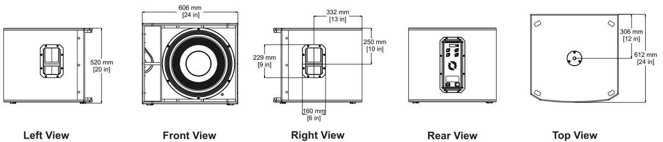
Figure 3.4: EKX-18SP dimensions
