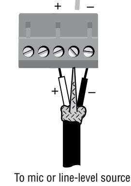
Figure 2.3 Mic/Line Connector
