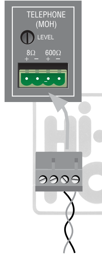
To telephone system interface/PBX input
